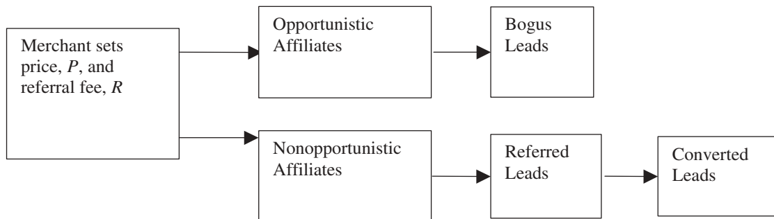
FIGURE 2 One-to-Many Model
